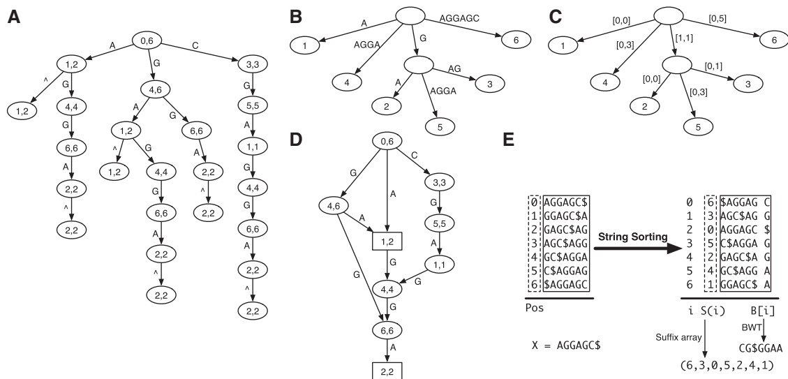
Figure 1: Data structures based on a prefix trie. (A) Prefix trie of string AGGAGC where symbol \hat{\phantom{a}} marks the start of the string. The two numbers in each node give the suffix array interval of the substring represented by the node, which is the string concatenation of edge symbols from the node to the root. (B) Compressed prefix trie by contracting nodes with in- and out-degree both being one. (C) Prefix tree by representing the substring on each edge as the interval on the original string. (D) Prefix directed word graph (prefix DAWG) created by collapsing nodes of the prefix trie with identical suffix array interval. (E) Constructing the suffix array and Burrows–Wheeler transform of AGGAGC. The dollar symbol marks the end of the string and is lexicographically smaller than all the other symbols. The suffix array interval of a substring W is the maximal interval in the suffix array with all suffixes in the interval having W as prefix. For example, the suffix array interval of AG is [1, 2]. The two suffixes in the interval are AGC$ and AGGAGC$, starting at position 3 and 0, respectively. They are the only suffixes that have AG as prefix.
