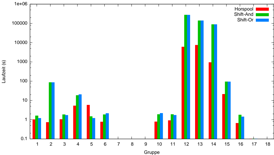
English Texts 1024MB (p="whatever")
