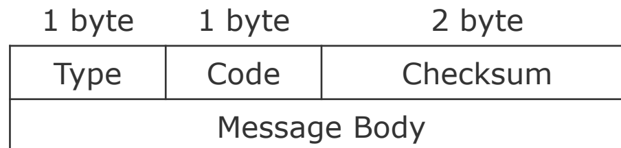
General format of ICMPv6 messages
