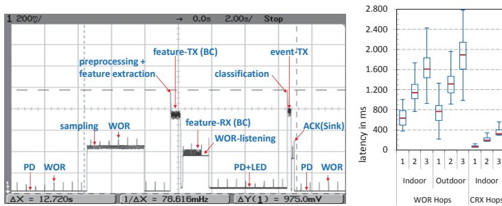
Fig. 8. Energy diagram for event processing
