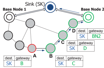
Fig. 6. Data transmission over base nodes to sink by using MMR
