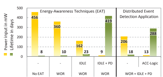
Fig. 10. Energy consumption and lifetime
