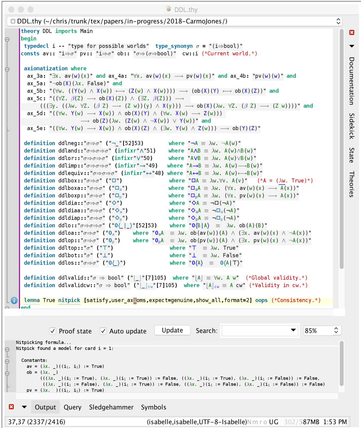
Figure 1: Shallow semantical embedding of DDL in Isabelle/HOL.
