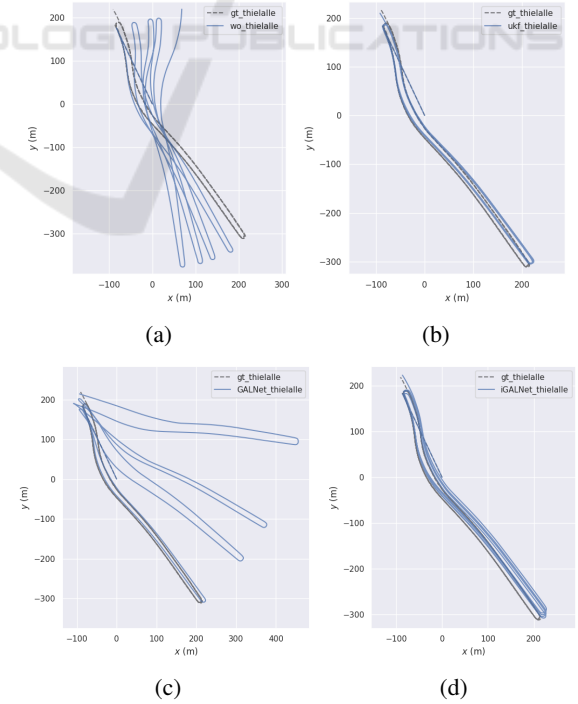
Figure 13: Resulting trajectories of the proposed methods in Thielallee. a) MIG wheel odometry, b) UKF wheel-inertial odometry, c) GALNet, d) iGALNet.
