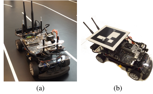
Figure 2: Developed (2018) Autominy TX1 version with odometry research purposes. a) Autominy TX1 on a track made with black rubber used to achieve aggressive driving manoeuvres, The ARUCO marker in b) is used to localize the car on the track.
