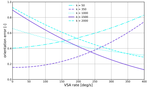
Figure 9: Orientation error for different values of \kappa related to the VSA rate ( \hat{\beta} ). Best values of \kappa for low and high \hat{\beta} are showed in purple.
