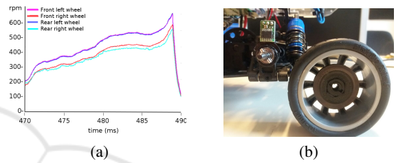
Figure 3: A) Wheel Angular Velocities of Autominy TX1. Front and rear left wheels have a bigger angular velocity since the car is driving on circles counterclockwise; when the car stops, velocities drop to zero. b) The Hall sensor mounted on the car chassis and the magnetic ring installed on the wheels.
