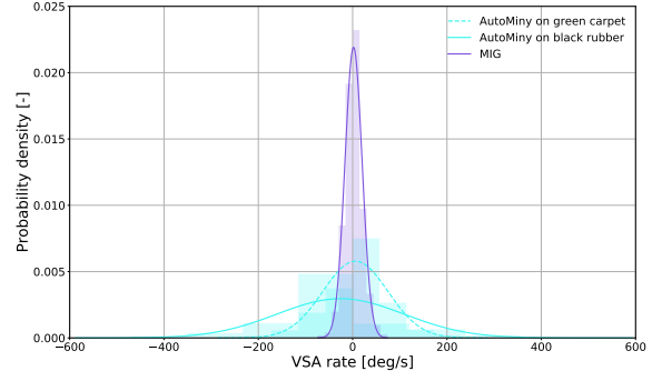
Figure 7: Range of VSA rates ( \beta ) in the datasets. Autominy developed higher \beta over black rubber, while as expected, the MIG performed the smallest values.
