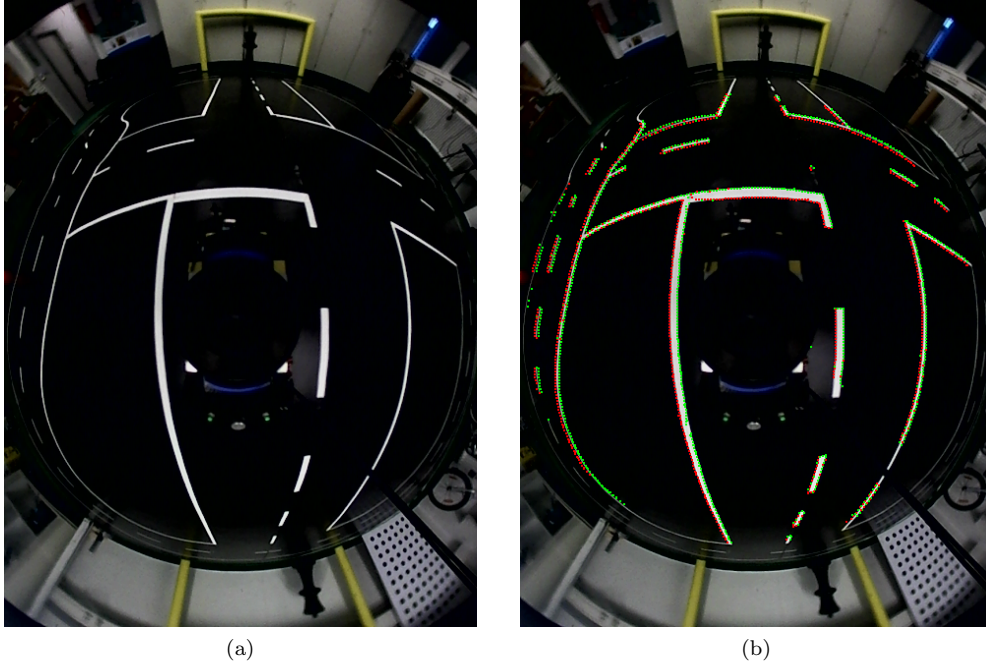
Figure 4.1: (a) shows an image from the omnidirectional camera, the found edgels are marked in (b).
