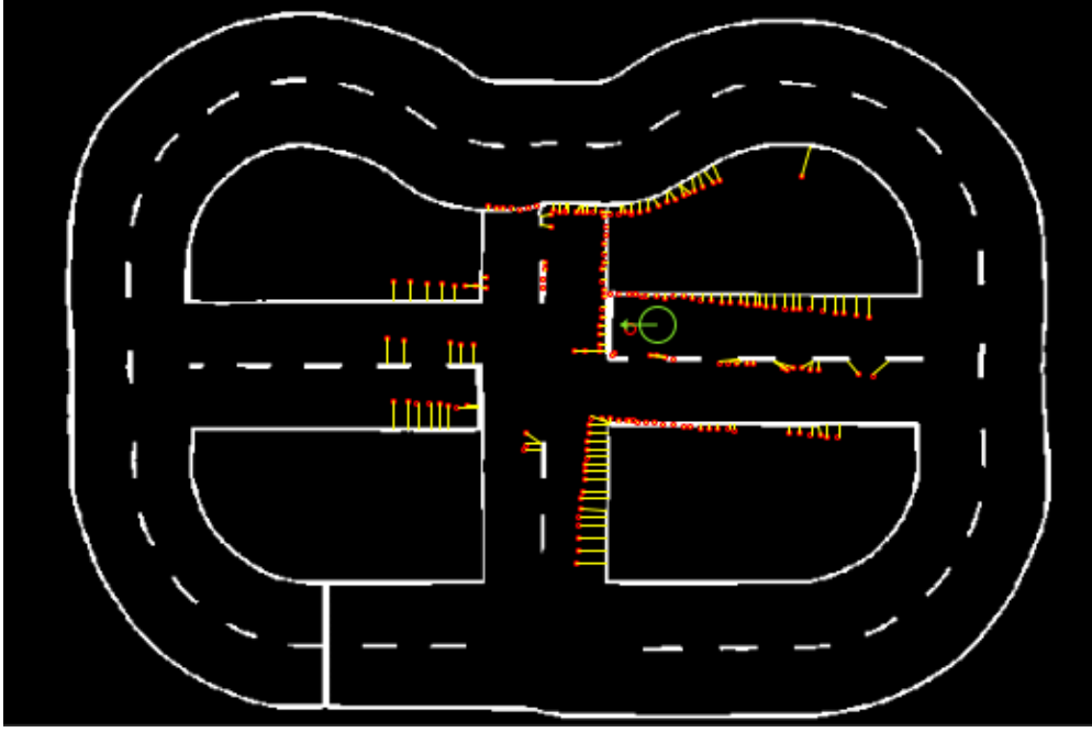
Figure 4.5: This shows an exaggerated example situation right before the correction step. The perception B from figure 4.2 (red) is transformed to the predicted pose estimate \bar{x} (green), where the force field \vec{F}_{NN} from figure 4.4.b exerts component forces (yellow) on the visible points from B_{\bar{x}} .
