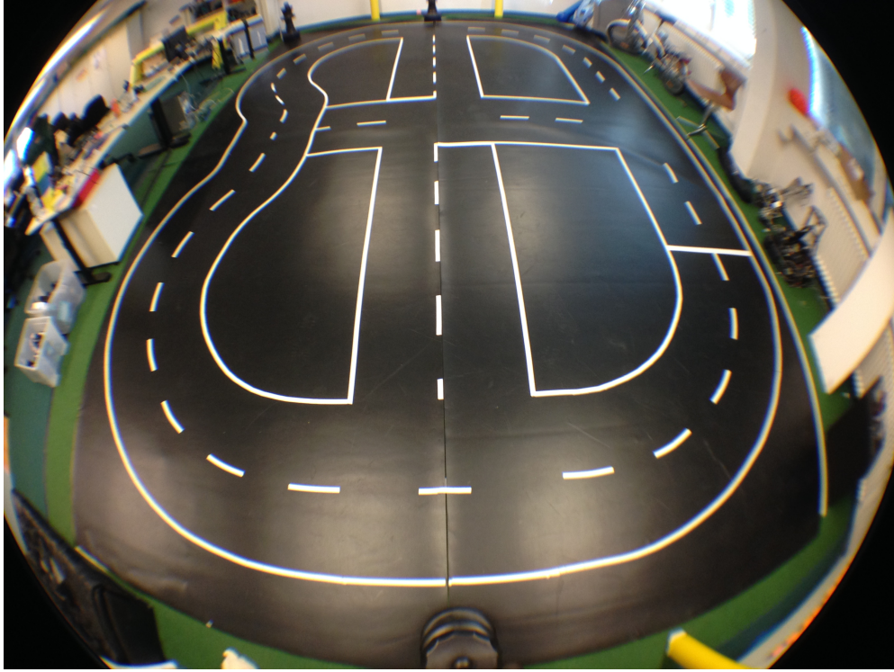
Figure 3.2: This is the test track in our lab, which is approximately 4 by 6 meters large. The reflections appear larger and more diffuse than from the car's perspective because the camera is further from the surface. We also shared this laboratory with the FUManoids team, so their test playing field is directly underneath the track. To the right, a line from their field is visible, which can erroneously be detected as a lane marker if not covered.
