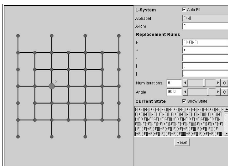
Fig. 10. JavaView applet to explore L-systems
