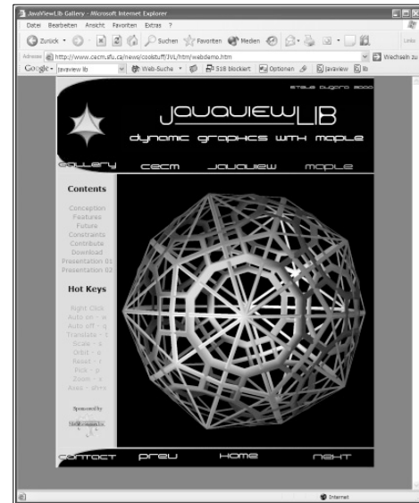
Fig. 2. Maple plot in JavaView
