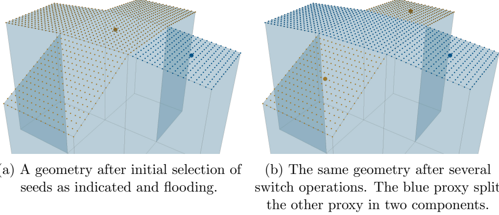
Figure 3: A proxy being torn apart by another proxy under the repeated application of the switch operation.
