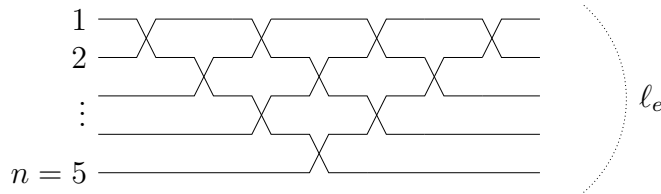
Fig. 4. The minimal element of B(5, 2)
