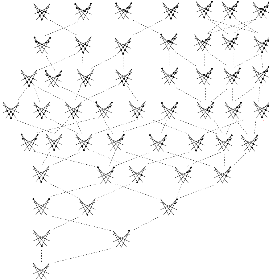
Fig. 9. A quarter of B(6,3) with the corresponding one element extensions of a cyclic line arrangement.
