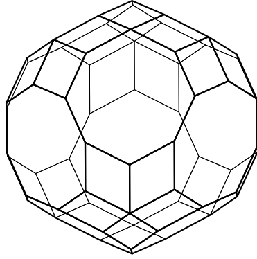
Fig. 3. The graph G_5 as graph of a zonotope.
