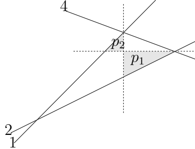
Fig. 7. The triangle of lines 1,2 and 4.
