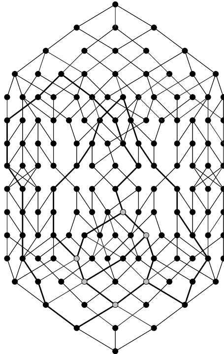
Fig. 8. The graph of B(6, 3) , with a highlighted subdivision of K_{3,3}
