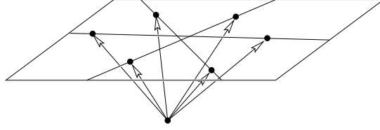
Fig. 5. The adjoint of C^{6,3} is not unique!
