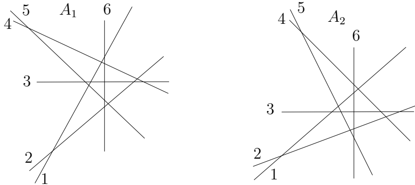
Fig. 6. Arrangements A_1 and A_2 .
