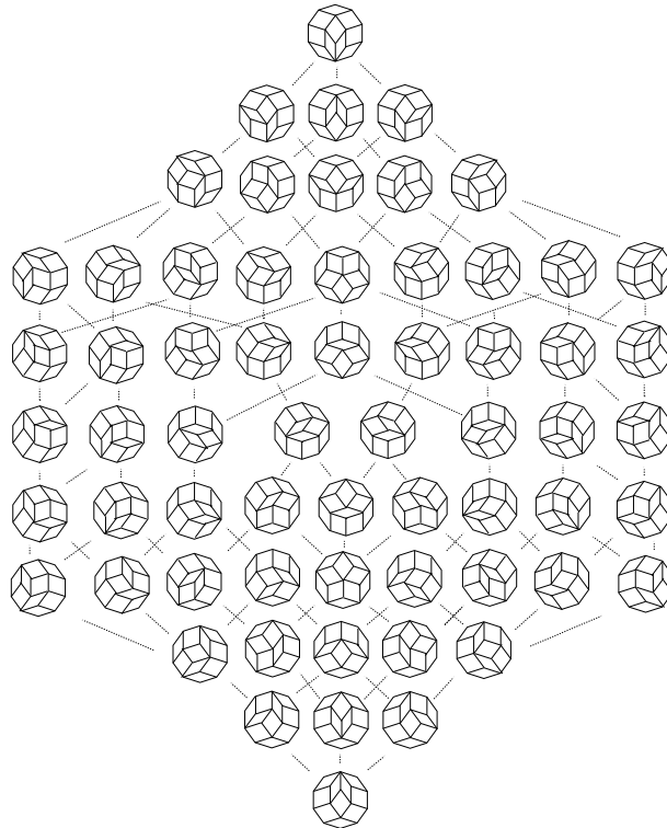
Fig. 2. The graph G_5 .
