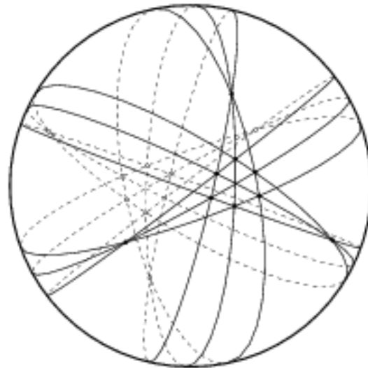
FIGURE 6.1.1 An arrangement of nine great circles on S^2 . The arrangement corresponds to a Pappus configuration.
