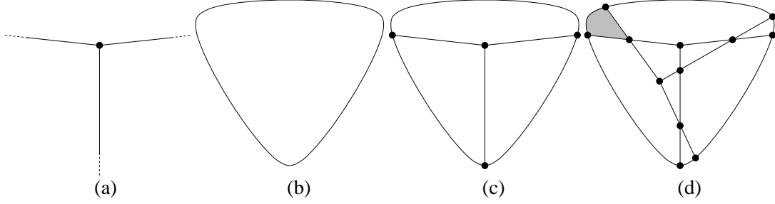
Figure 7: A part of the normal fan over the vertex \tau_{12} of Q (a), over \sigma_{123} (b), over the corresponding edge \sigma_{12} (c), and over the adjacent 2-dimensional chamber \sigma_1 (d). If \psi_{\sigma_1} is chosen in the interior of the shaded cone, and if \psi_{\sigma_2} and \psi_{\sigma_3} are chosen analogously with respect to the rotational symmetry we get the basket ball obstruction of Figure 6.
