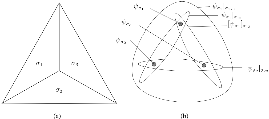
Figure 5: A really simple chamber complex (a) and a sketch for a possible “locally coherent” choice of function values on this complex (b).
