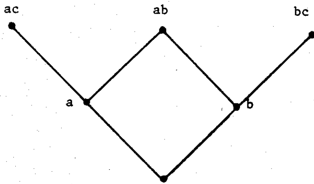
undirected branching greedoid of G
