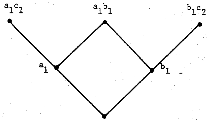
branching greedoid of D(G)
