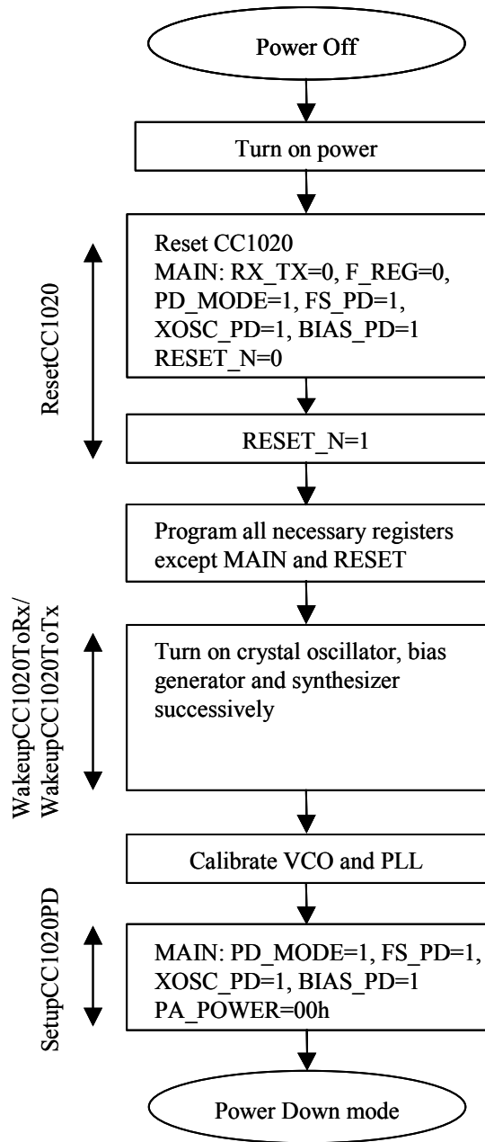
Figure 30. Initialising sequence
