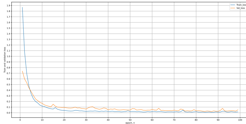
Figure 23: Plot of training and validation loss with large weight decay of Adam optimizer.
