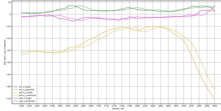
Figure 21: Outputs of LSTM1 model on dataset with flipped negative quaternions for roll, pitch, yaw axes.
