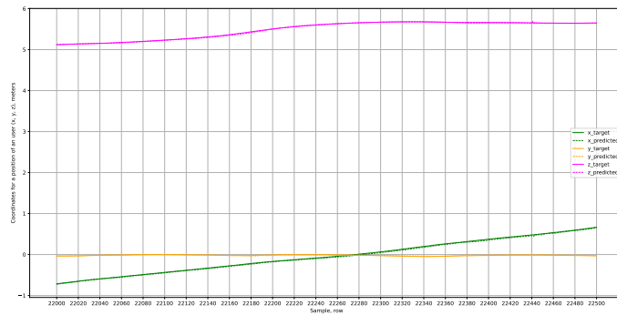
Figure 30: GRU1 outputs for position (x, y, z) for rows 22000..22500.
