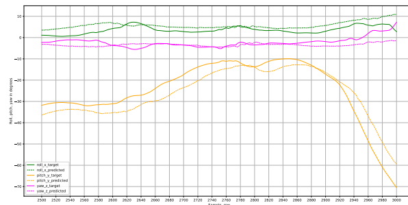
Figure 32: Bidirectional GRU outputs for roll, pitch, yaw axes.
