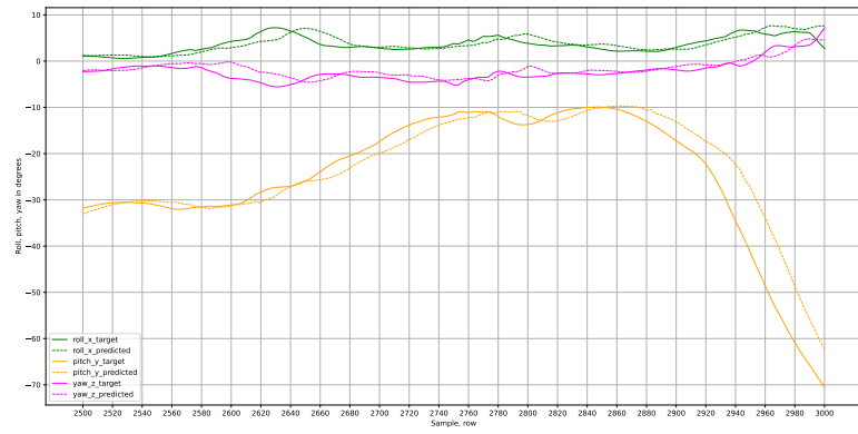
Figure 19: Outputs of LSTM1 model on interpolated dataset for roll, pitch, yaw axes.
