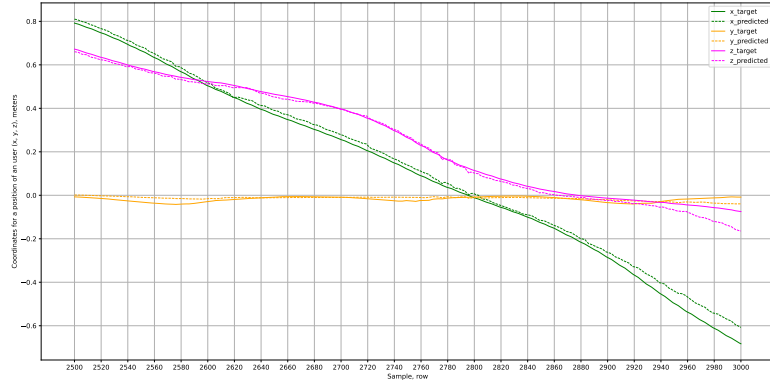
Figure 24: Outputs of LSTM2 model with ReLU activation function for x, y and z axes.
