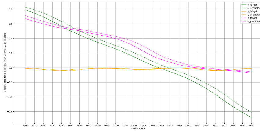
Figure 15: Outputs of Baseline Model for x, y and z axes.
