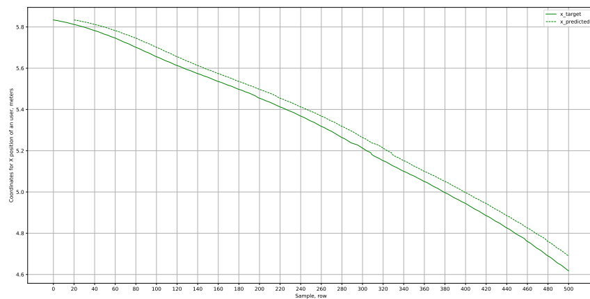
Figure 14: Outputs of Baseline Model for x-axis.
