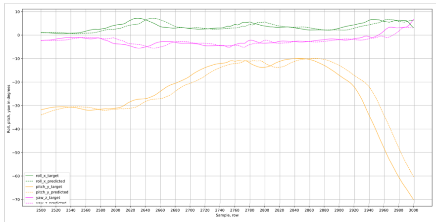
Figure 17: Outputs of Baseline Model for rotation data represented as Euler angles.
