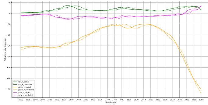
Figure 31: GRU1 outputs for roll, pitch, yaw axes.
