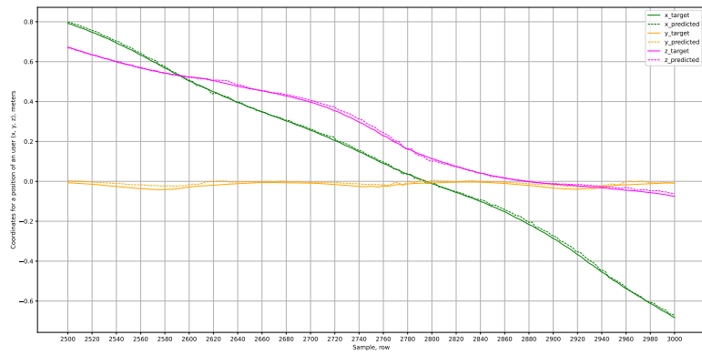
Figure 20: Outputs of LSTM1 model on dataset with flipped negative quaternions for x, y and z axes.
