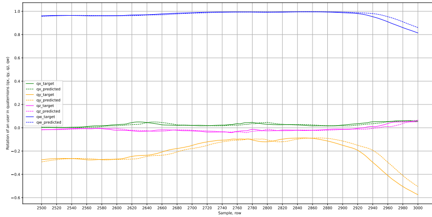
Figure 16: Outputs of Baseline Model for quaternions components qx, qy, qz and qw.
