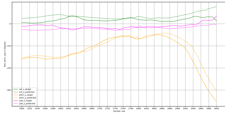
Figure 25: Outputs of LSTM2 model with ReLU activation function for roll, pitch, yaw axes.
