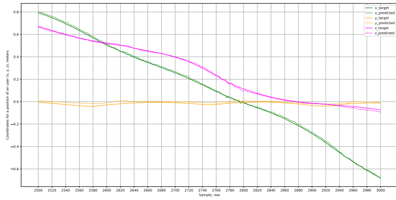
Figure 18: Outputs of LSTM1 model on interpolated dataset for x, y and z axes.
