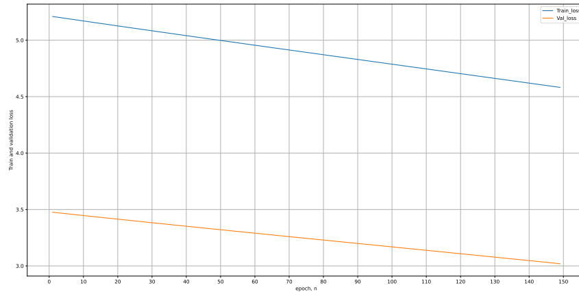
Figure 22: Plot of training and validation loss with small learning rate of Adam optimizer.
