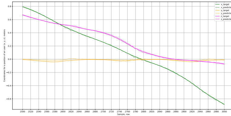
Figure 26: Outputs of LSTM3 model with Mish activation function for x, y and z axes.
