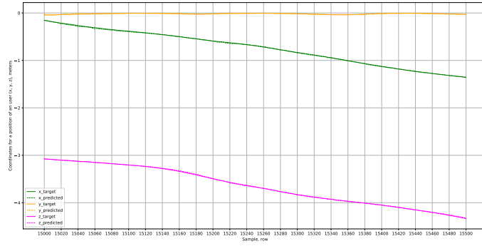
Figure 29: GRU1 outputs for position (x, y, z) for rows 15000..15500.
