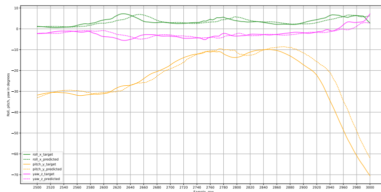
Figure 27: Outputs of LSTM3 model with Mish activation function for roll, pitch, yaw axes.
